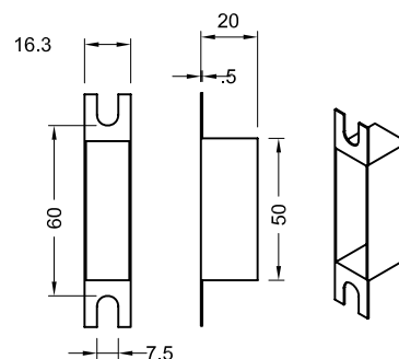
Keeper Cup
