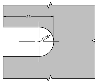
Glass Preparation
