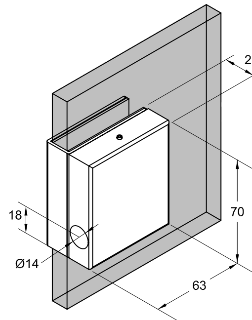
GK629
