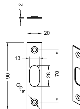
Keeper Plate
