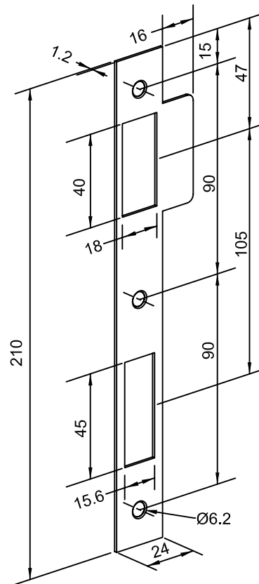
Strike Plate
