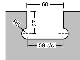
Glass Preparation (US631 / GK631 )
