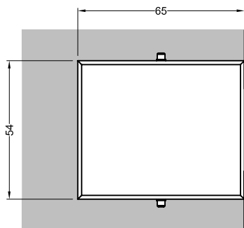
GK623 (NEW)
