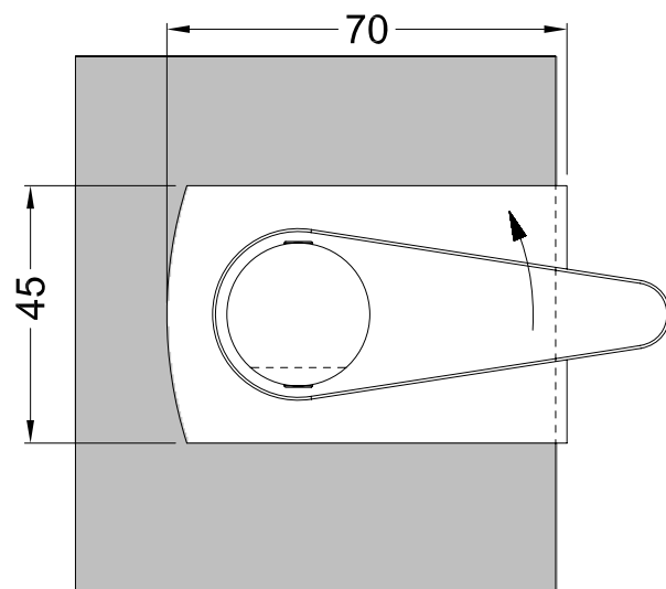
US624 Latch
