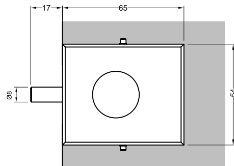
US623 (NEW)
