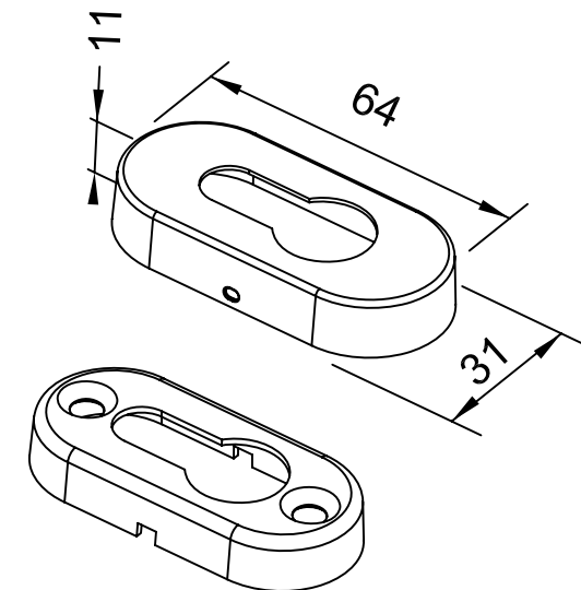
Covers for Key Cylinder (2 sets )
