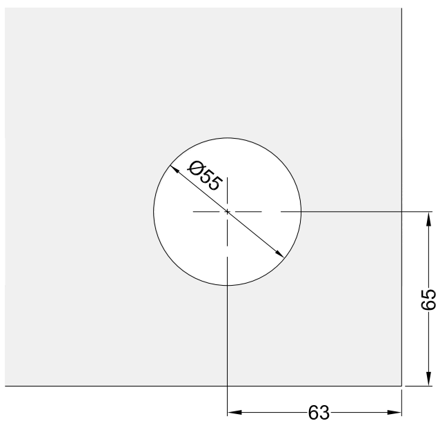
Glass Preparation for Swing Door
