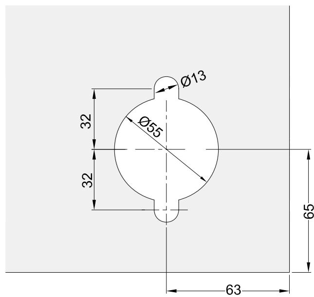
Glass Preparation for Sliding Door
