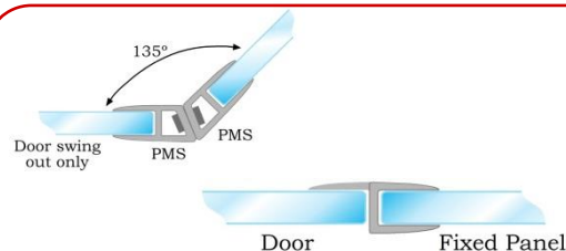
Vinyl Clip Seals – Deane Series
