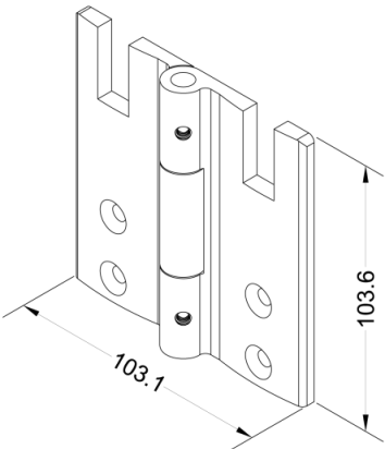
HN100 – Hinge (DRM100)
