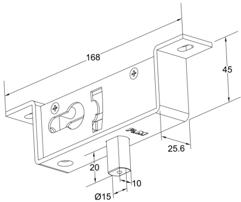
PL2 – Lock Bolt
