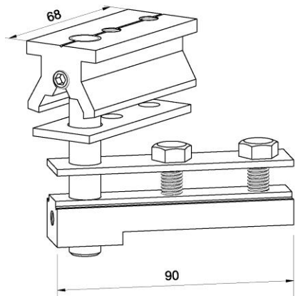
400TP – Top Pivot with Slider
