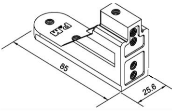
HN810 – Bracket
