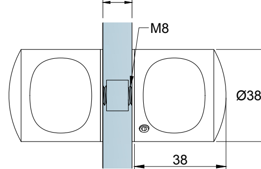
KH16 Ø38 Door Knob
