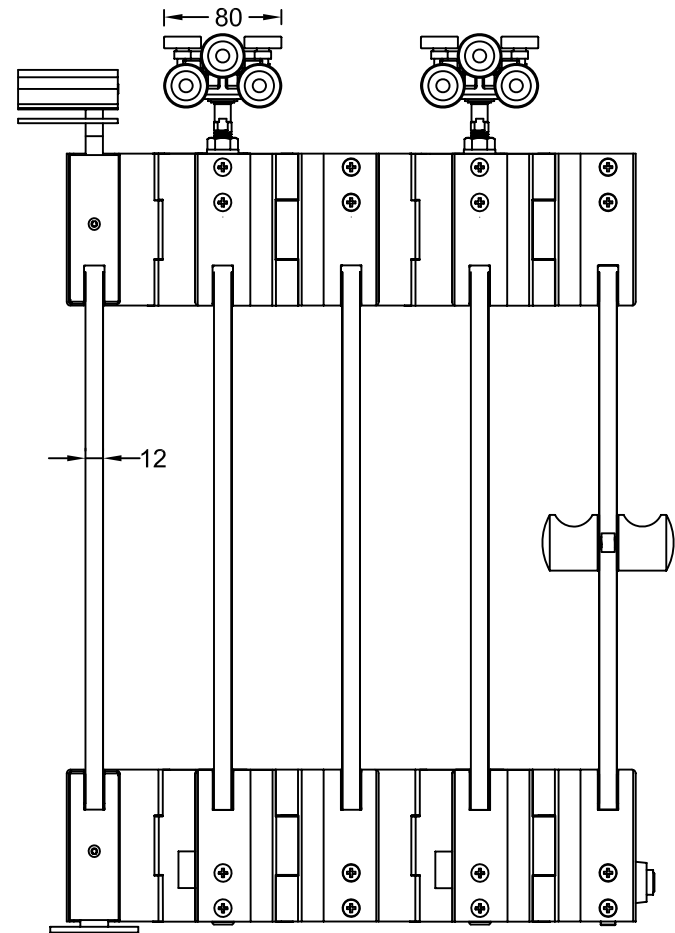
END VIEW
