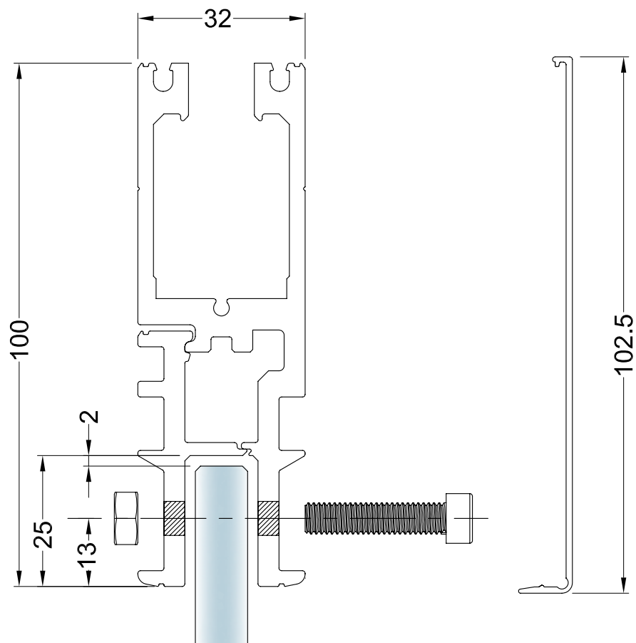
SLF400 Top Rails Extrusions
