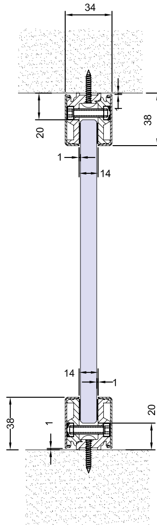
DRM38 Fixed Panel Rails
