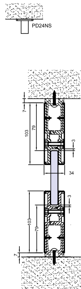
DRM100 Fixed Panel Rails
