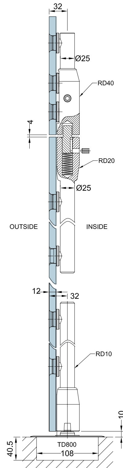
CROSS SECTION
