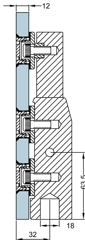
SECTION B-B
