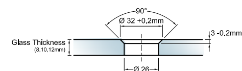
Glass Preparation for Countersunk Point Stud
