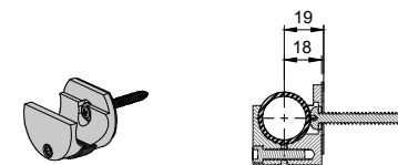
MTDOS-TTW Track to Wall Fixing
