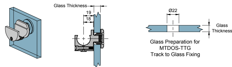
MTDOS-TTG Track to Glass Fixing
