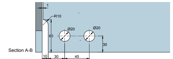
Glass Preparation for Fin Fitting Attachment Panel
