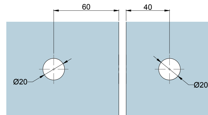
Glass Preparation (19mm Glass Thickness)
