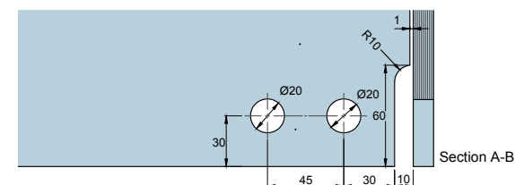
Glass Preparation for Fin Fitting Attachment Panel
