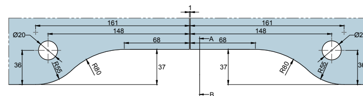
Glass Preparation for Overpanel
