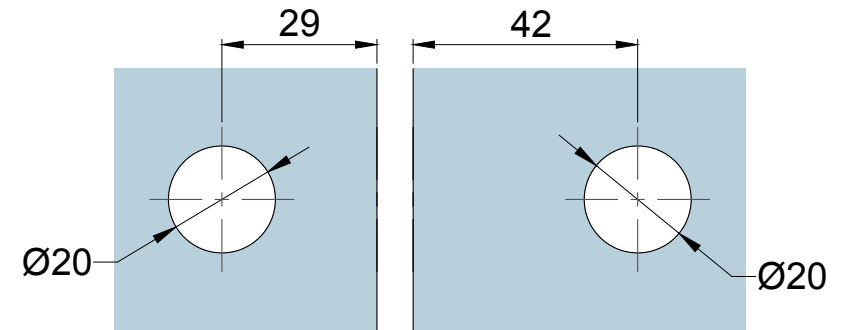
Glass Preparation (12mm Glass Thickness)
