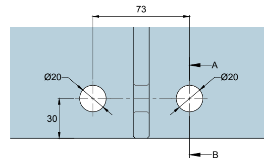
Glass Preparation for Overpanel
