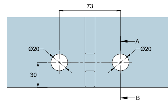
Glass Preparation for Overpanel
