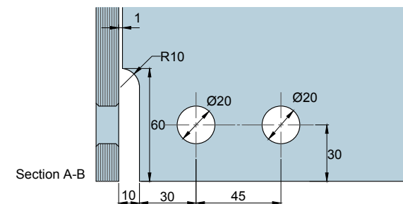
Glass Preparation for Fin Fitting Attachment Panel
