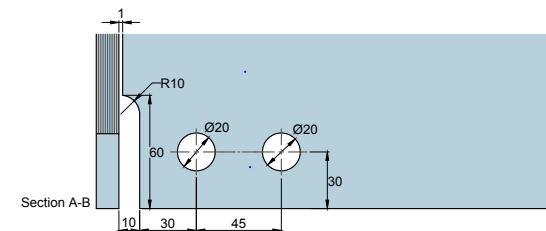
Glass Preparation for Fin Fitting Attachment Panel
