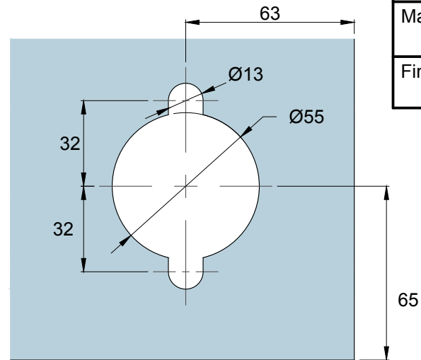
Glass Preparation for Sliding Door
