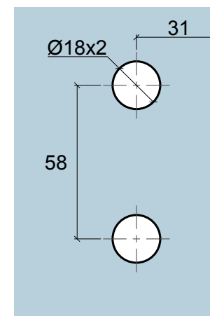
Glass Preparation for Fixed Panel
