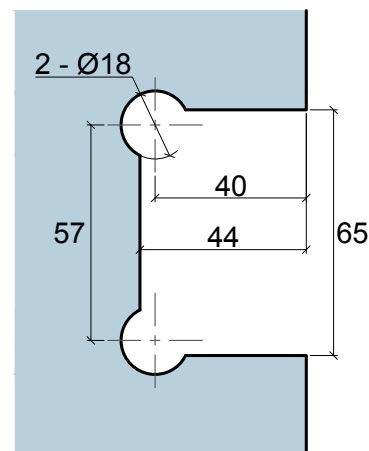
Glass Preparation for Door Panel
