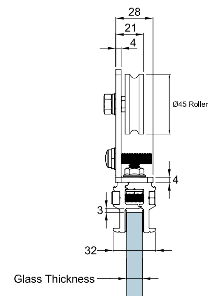
SC60 Hanger with Roller and SF-AC94 200mm Glass Clamp (Side Elevation)
