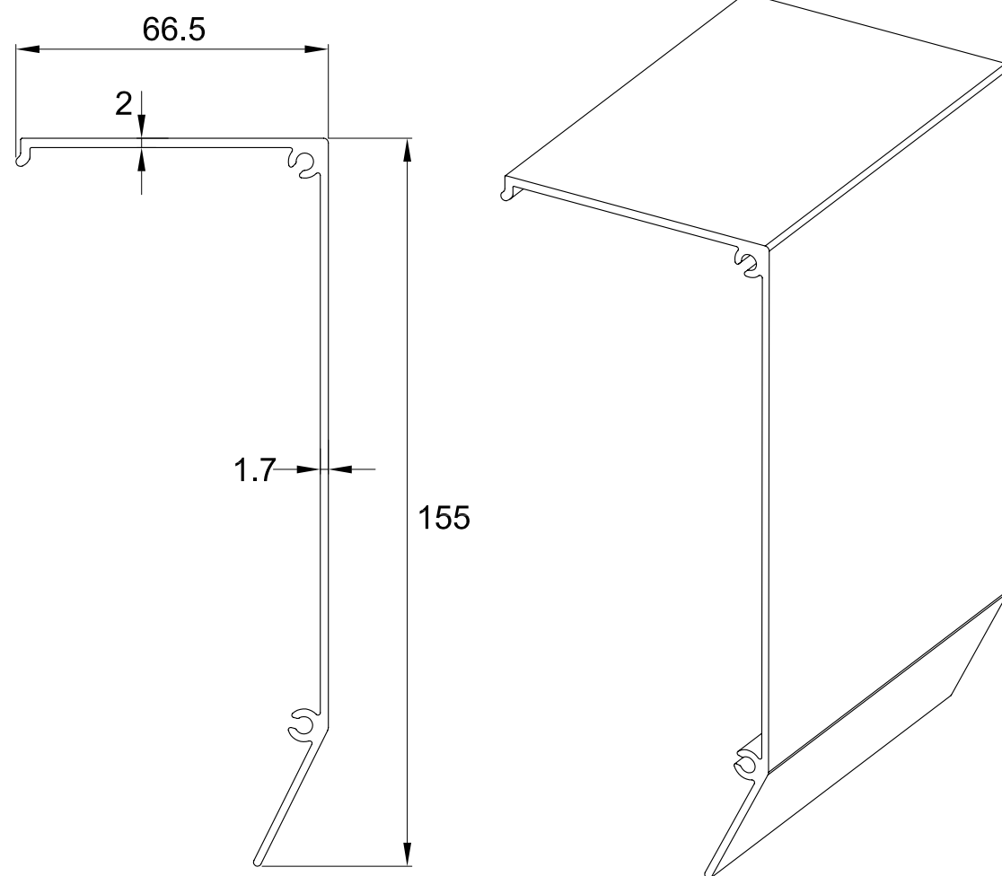
Flip on Cover
