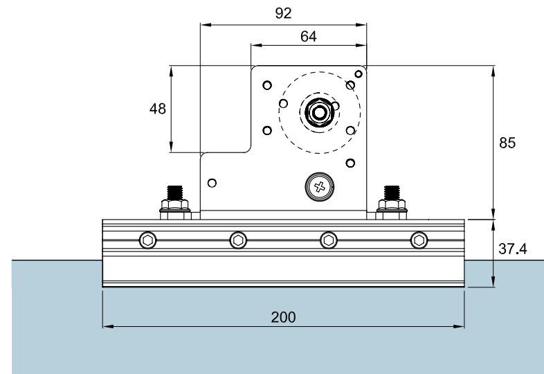
SC60 H-B Hanger with Roller and SF-AC94 200mm Glass Clamp (Front Elevation)
