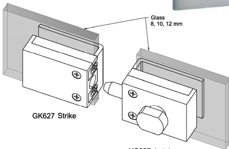
US627 Latch
