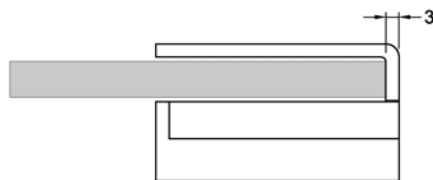
US627 Latch
