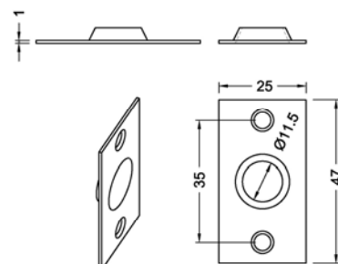
Keeper Plate
