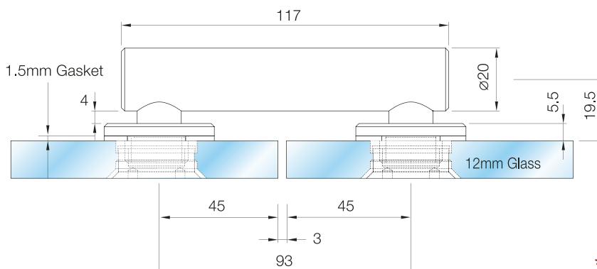
MC2 180° Glass to Glass Connector
