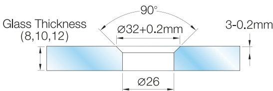
Glass Preparation for Countersunk Point Stud
