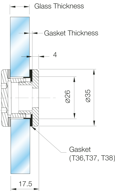
FHA-Flathead Point Stud (Adjustable)
