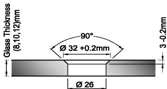
Glass Preparation for Countersunk Point Stud
