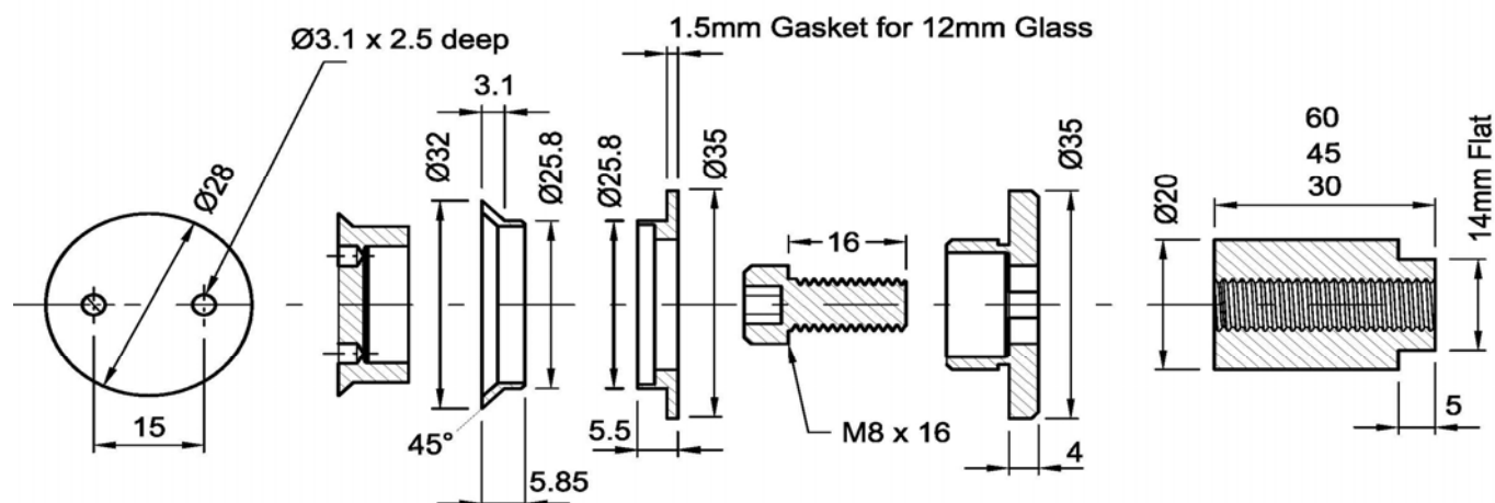
Glass Preparation for Countersunk Point Stud
